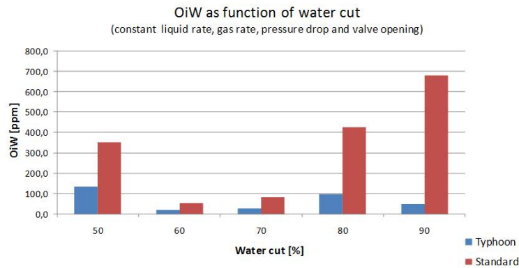
Figure 6: Separator water outlet OiW concentration as a function of WC and valve type (left), water samples from the same test conditions for the standard and Typhoon Valve System (right).
